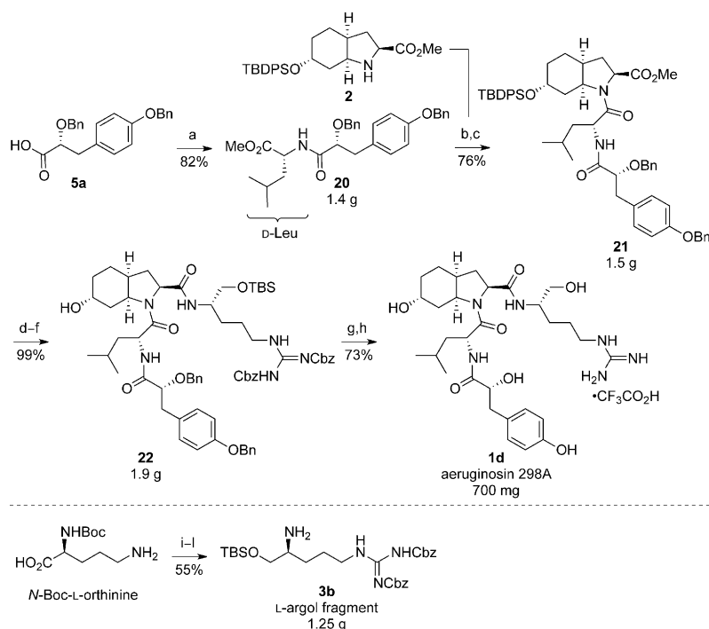
Scheme 5. Synthesis of aeruginosin 298A ( 1d ). Reagents and conditions: a) D-Leu-OMe, PyBOP, i\text{Pr}_2\text{NEt} , \text{CH}_2\text{Cl}_2 , 20°C, 82%; b) LiOH, THF/MeOH (3:1), 0→20°C; c) 2 (1.2 equiv), PyBOP, i\text{Pr}_2\text{NEt} , \text{CH}_2\text{Cl}_2 , 20°C, 76% for 2 steps; d) HF-pyridine, \text{CH}_3\text{CN} , 0°C, 99%; e) LiOH, THF/MeOH (2:1), 0→20°C; f) 3b (1.2 equiv), HBTU, i\text{Pr}_2\text{NEt} , DMF, 0→20°C, quant. for 2 steps; g) HCl (0.5%), MeOH, 0°C, 78%; h) \text{H}_2 , \text{Pd}(\text{OH})_2/\text{C} , MeOH/AcOEt (1:1), 20°C, then \text{CF}_3\text{CO}_2\text{H} , 93%; i) \text{TFN}=\text{C}(\text{NHCCbz})_2 , \text{CF}_3\text{C}(\text{=O})\text{N}(\text{Me})\text{SiMe}_3 , \text{Et}_3\text{N} , \text{CH}_2\text{Cl}_2 , 20°C, 76%; j) isobutyl chloroformate, N -methylmorpholine, THF, −10°C, then \text{NaBH}_4 , THF/ \text{H}_2\text{O} (4:1), 0→20°C, 74%; k) TBSCl, imidazole, \text{CH}_2\text{Cl}_2 , 0→20°C, 99%; l) TMSOTf, 2,6-lutidine, \text{CH}_2\text{Cl}_2 , −78→20°C, 100%. TMS = trimethylsilyl.
