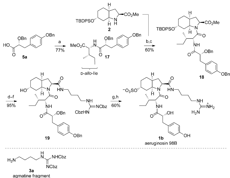
Scheme 4. Synthesis of aeruginosin 98B ( 1b ). Reagents and conditions: a) D-allo-Ile-OMe, PyBOP, i Pr 2 NEt, CH 2 Cl 2 , 20 °C, 77%; b) LiOH, THF/MeOH 3:1, 0 → 20 °C; c) 2 (1.2 equiv), PyBOP, i Pr 2 NEt, CH 2 Cl 2 , 20 °C, 60% for 2 steps; d) HF-pyridine, CH 3 CN, 0 °C, 95%; e) LiOH, THF/MeOH (2:1), 0 → 20 °C; f) 3a (1.2 equiv), HBTU, i Pr 2 NEt, DMF, 0 → 20 °C, 100% for 2 steps; g) SO 3 ·pyridine, pyridine, 50 °C; h) H 2 , Pd(OH) 2 /C, MeOH/AcOEt (1:1), 20 °C, 60% for 2 steps. PyBOP = (benzotriazol-1-yloxy)tripyrrolidino-phosphonium hexafluorophosphate, THF = tetrahydrofuran.
